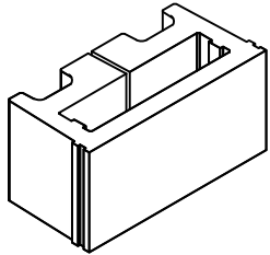
ISOMETRIC
